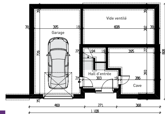
Plan MC300 by DOMUS CONCEPT
