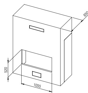
INSTALLATION WITH RECESSED CLADDING KIT K0069AZ00
