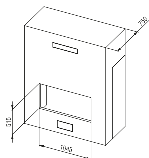
INSTALLATION WITH CLADDING PROVIDED BY THE FACTORY
