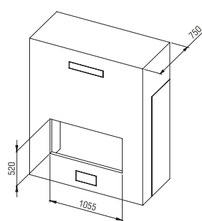
4 SIDES CLADDING INSTALLATION KIT K0066AZ00
