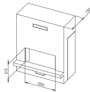
3 SIDES CLADDING INSTALLATION KIT K0067AZ00
